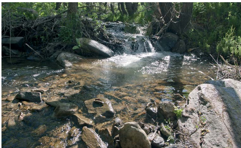
Fig. 5: Stream No. 1, southwest of Lake Van, east Turkey, in which numerous Neurergus strauchii (STEINDACHNER, 1887) were found.
